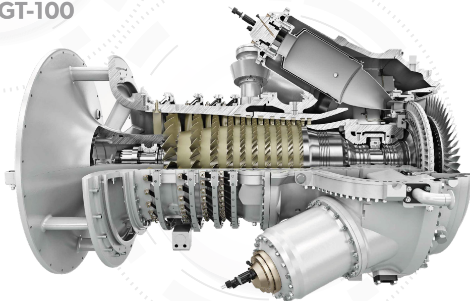
Industrial gas turbine SGT-300
