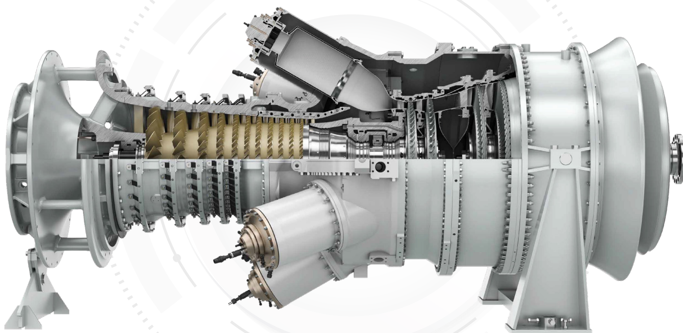
Industrial gas turbine SGT-400
