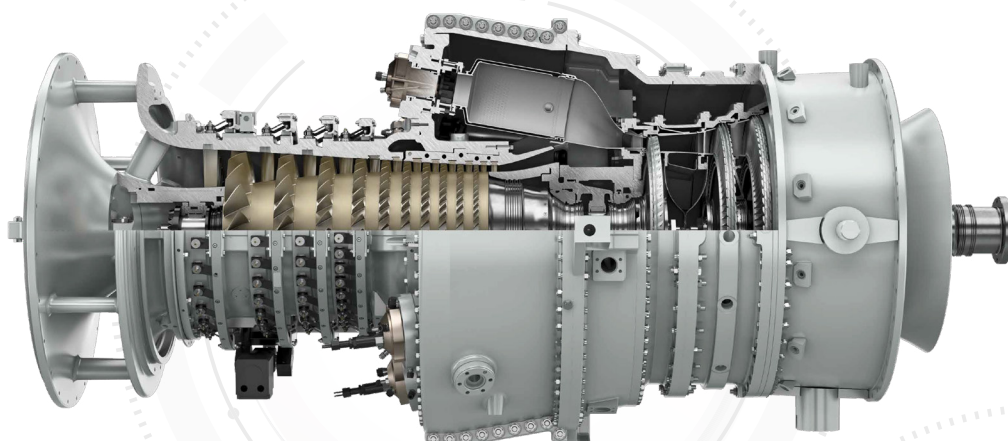
Industrial gas turbine SGT-100
